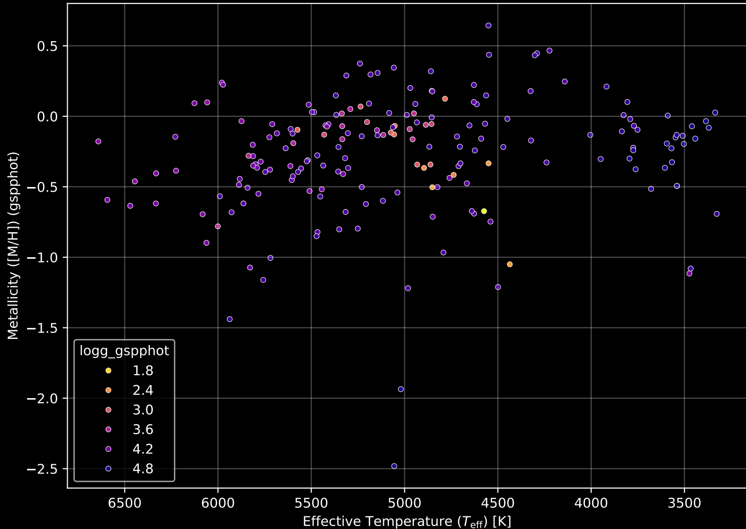
APOGEE DR17 Field: [K2_C8_123-53] Stellar Population Parameters (n= 192)
