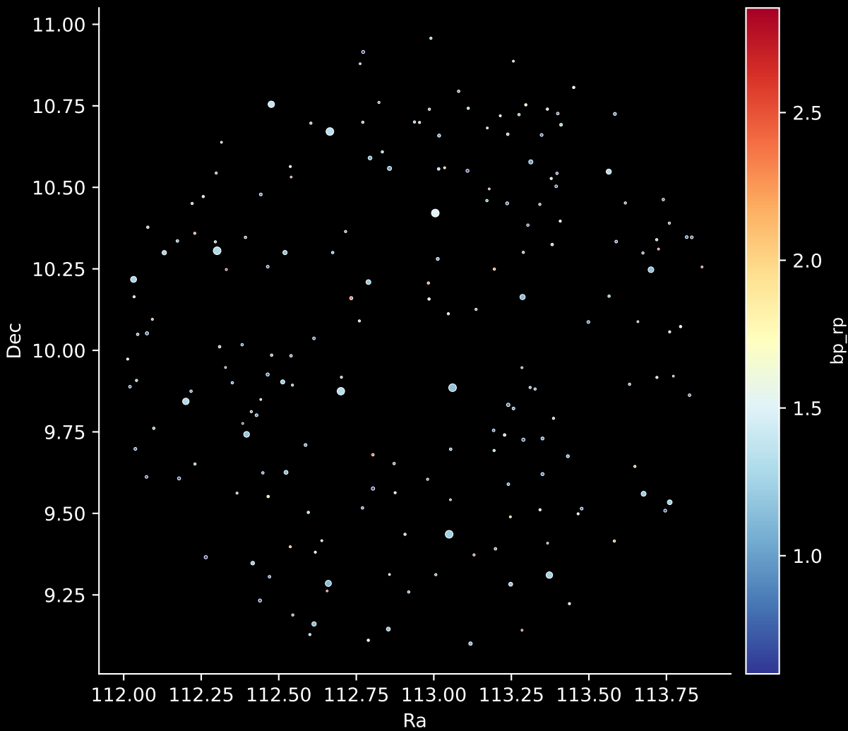
APOGEE DR17 Field: [K2_C8_123-53] Stars: 192
