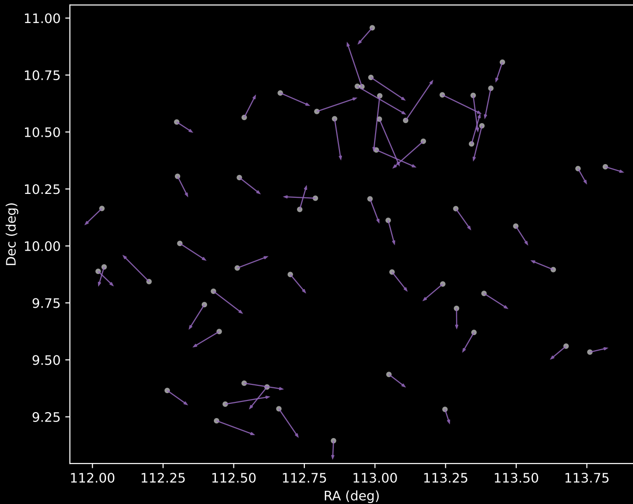
APOGEE DR17 Cluster 8 Proper Motion Vectors (n=57)
