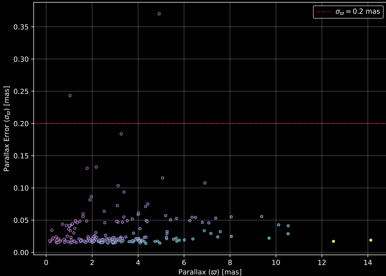
APOGEE DR17 Field: [K2_C8_123-53] Parallax Quality (n= 192)
