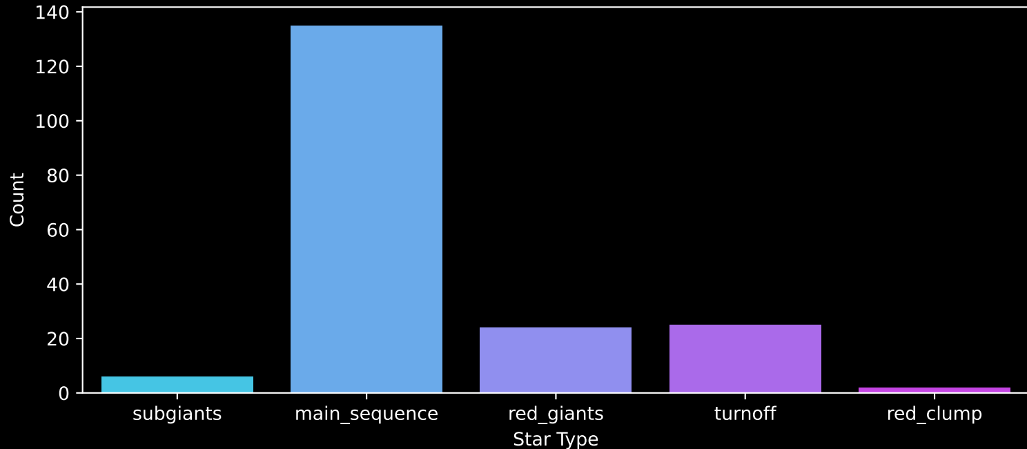
APOGEE DR17 Field: [K2_C8_123-53] Count plot of Star Type
