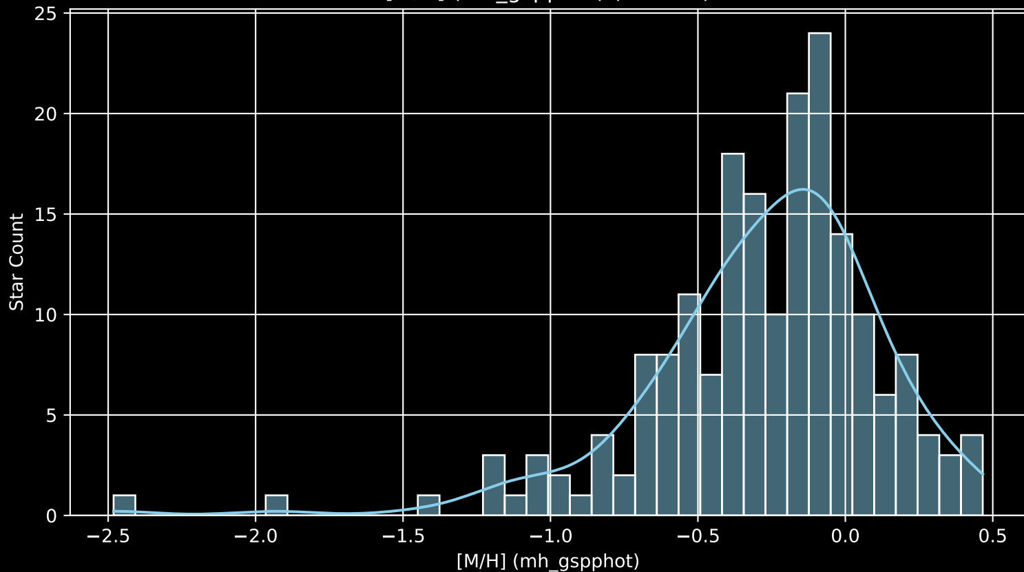
APOGEE DR17 Field: [K2_C8_123-53 [M/H] (mh_gspphot) (n= 191)
