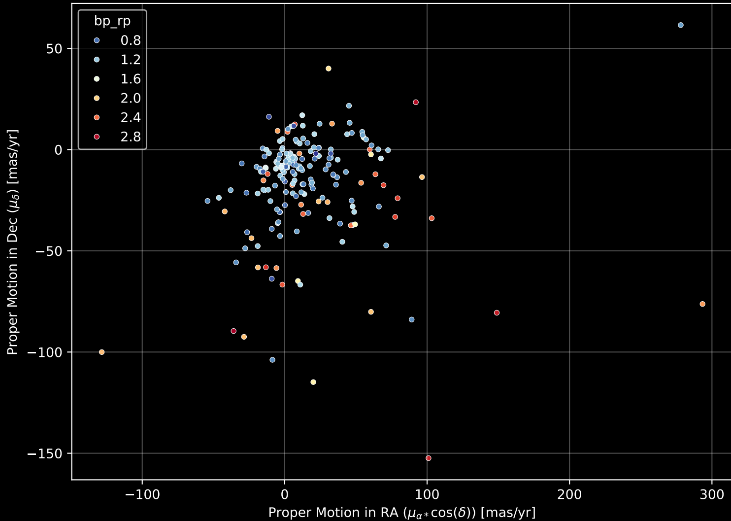
APOGEE DR17 Field: [K2_C8_123-53] Proper Motion Diagram (n= 192)
