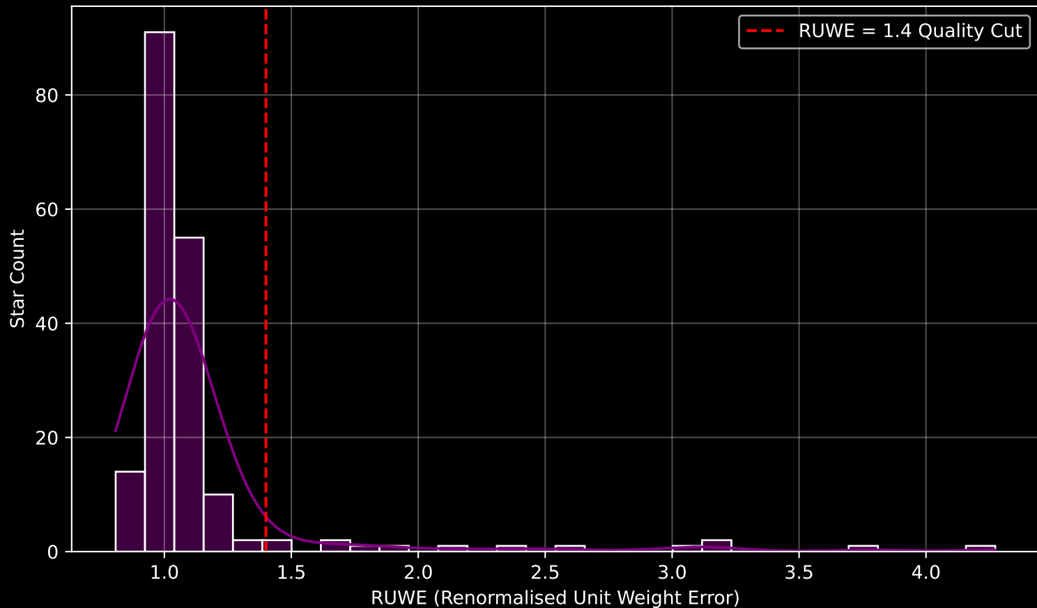
GAPOGEE DR17 Field [K2_C8_123-53] RUWE Distribution (n= 186)
